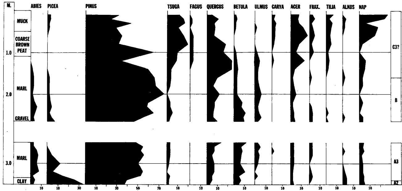
FIGURE 4. Pollen diagram at sites IIA and IIB, Savannah.
