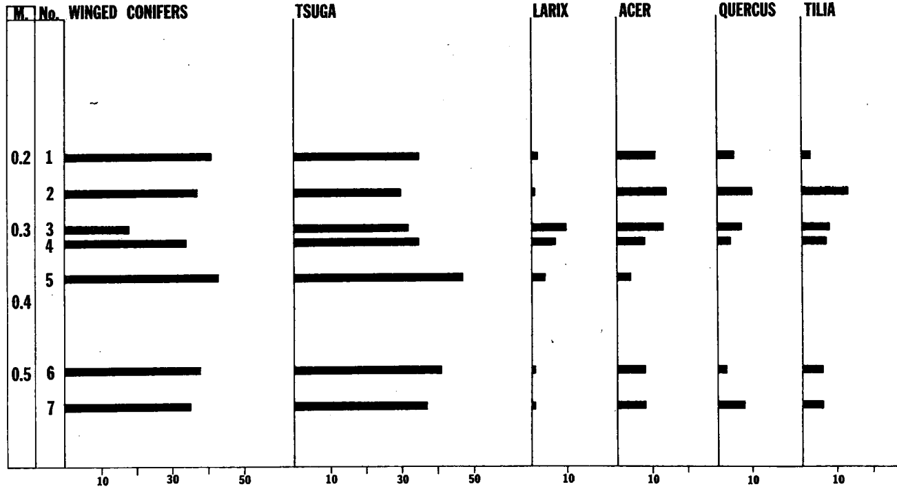
FIGURE 7. Pollen diagram constructed from the seven samples taken from the archeological test pit at site II. Percentages based on total arboreal pollen.
