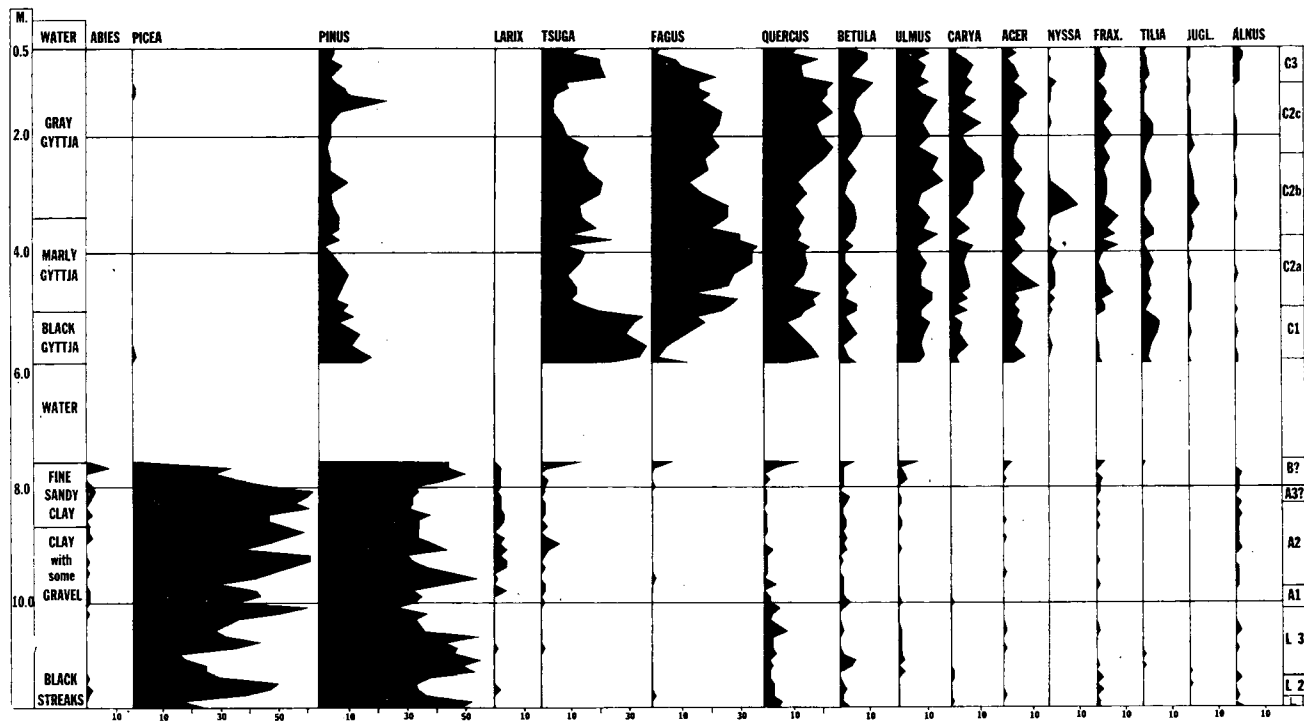
FIGURE 2. Arboreal pollen diagram at site I, Crusoe Lake.
