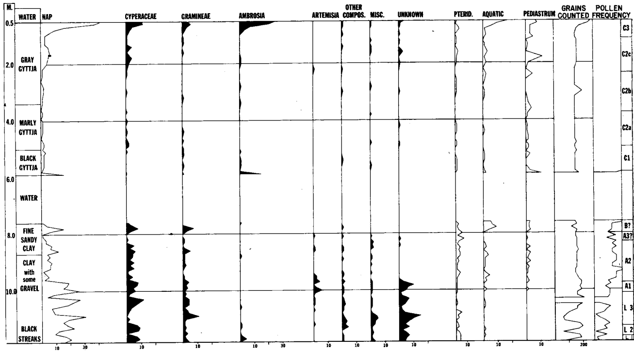
FIGURE 3. Nonarboreal pollen diagram at site I, Crusoe Lake.
